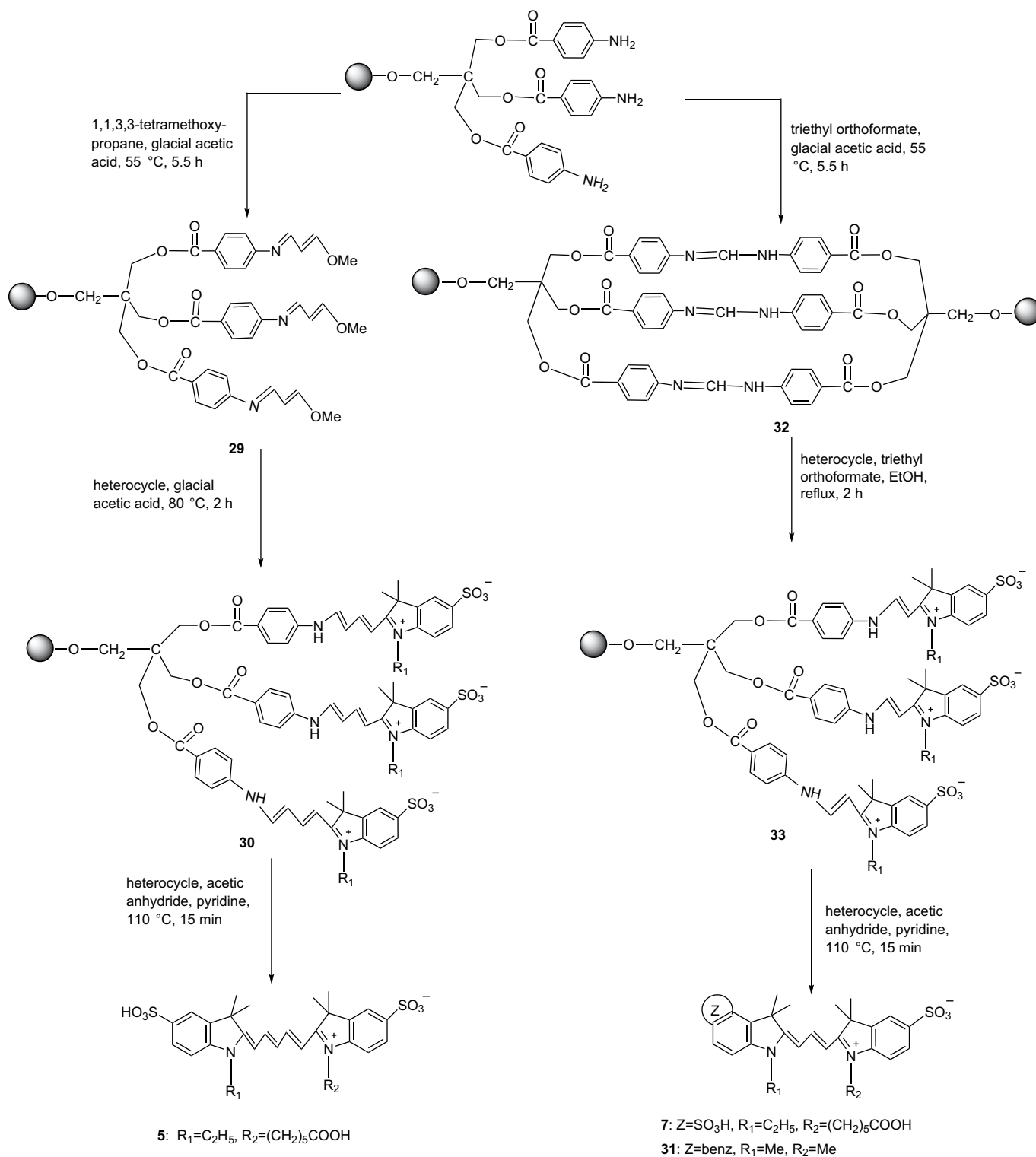
Scheme 7. Synthesis of water-soluble cyanine dyes by using PEG-(PhNH 2 ) 6 as a support.
