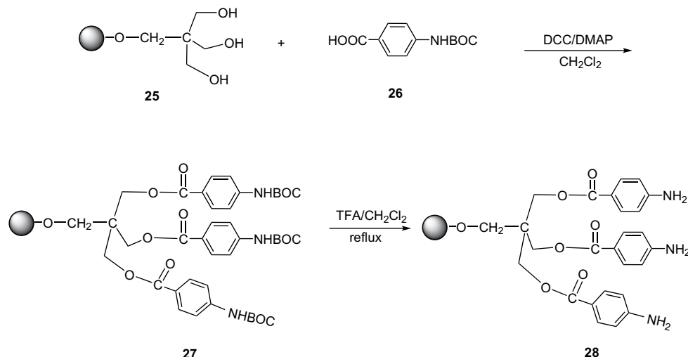
Scheme 6. Synthetic procedure of PEG-(PhNH 2 ) 6 .
