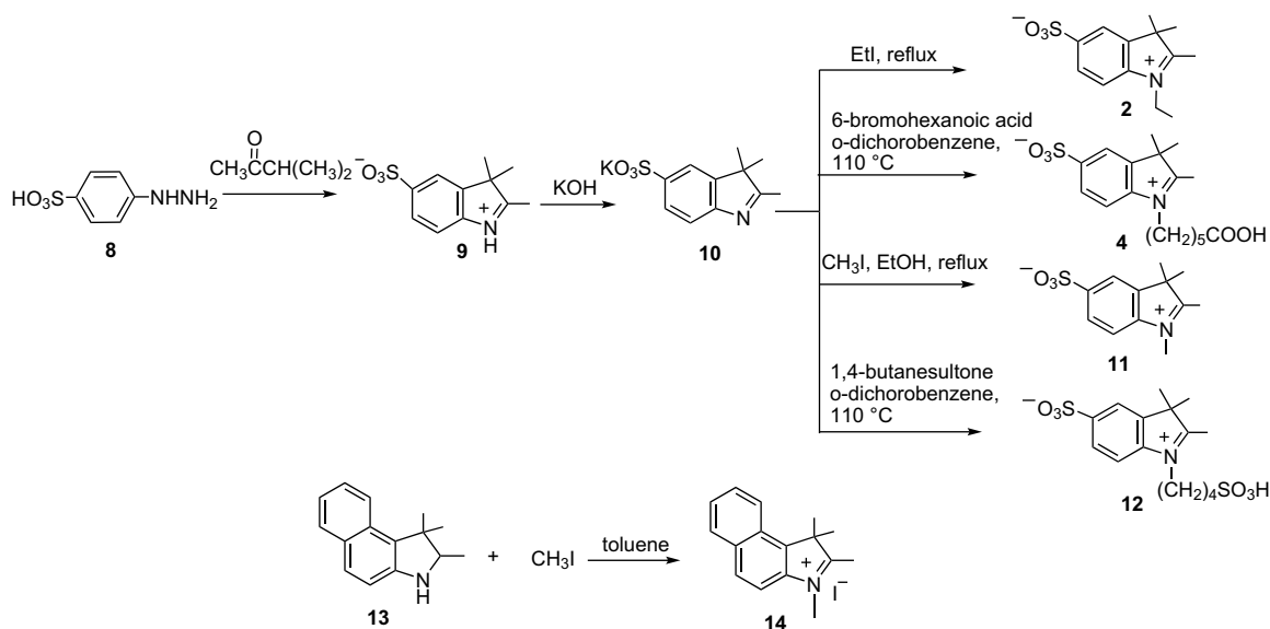
Scheme 3. Synthesis of heterocycle compounds.
