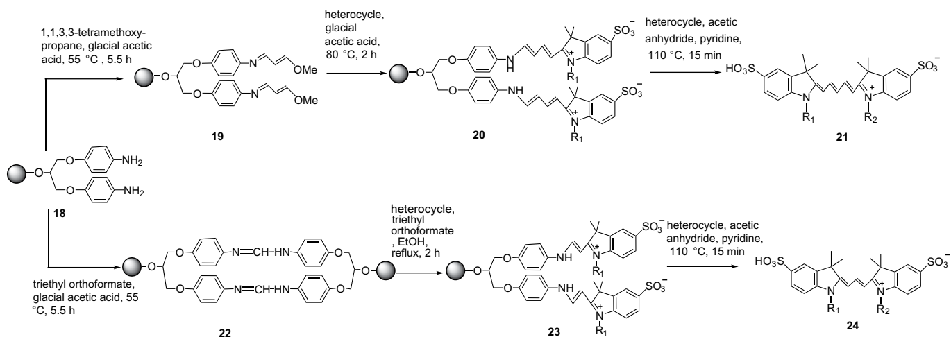
Scheme 5. PEG-(PhNH 2 ) 4 supported synthesis of unsymmetrical water-soluble cyanine dyes.
