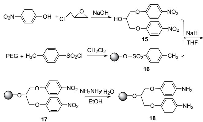
Scheme 4. Synthesis of PEG-(PhNH 2 ) 4 .
