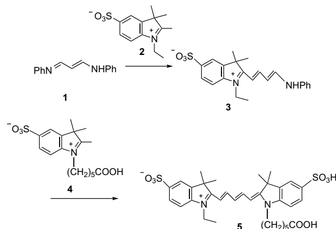
Scheme 1. Traditional synthesis of a water-soluble cyanine dye.
