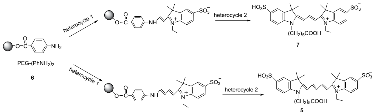
Scheme 2. Synthesis of cyanine dyes by using PEG-(PhNH 2 ) 2 support.
